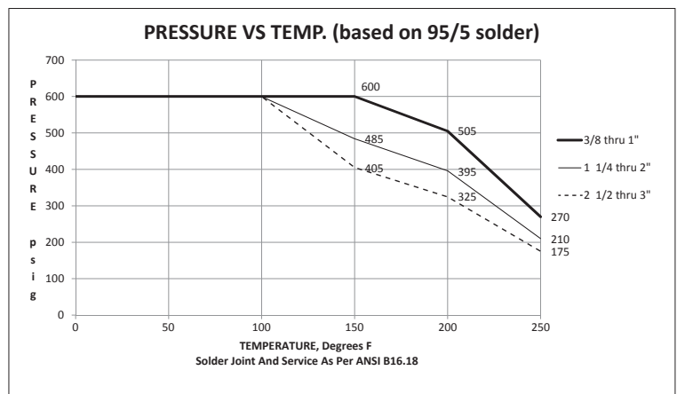
PRESSURE - TEMPERATURE CHART VACUUM SERVICE TO 29 INCHES Hg.
